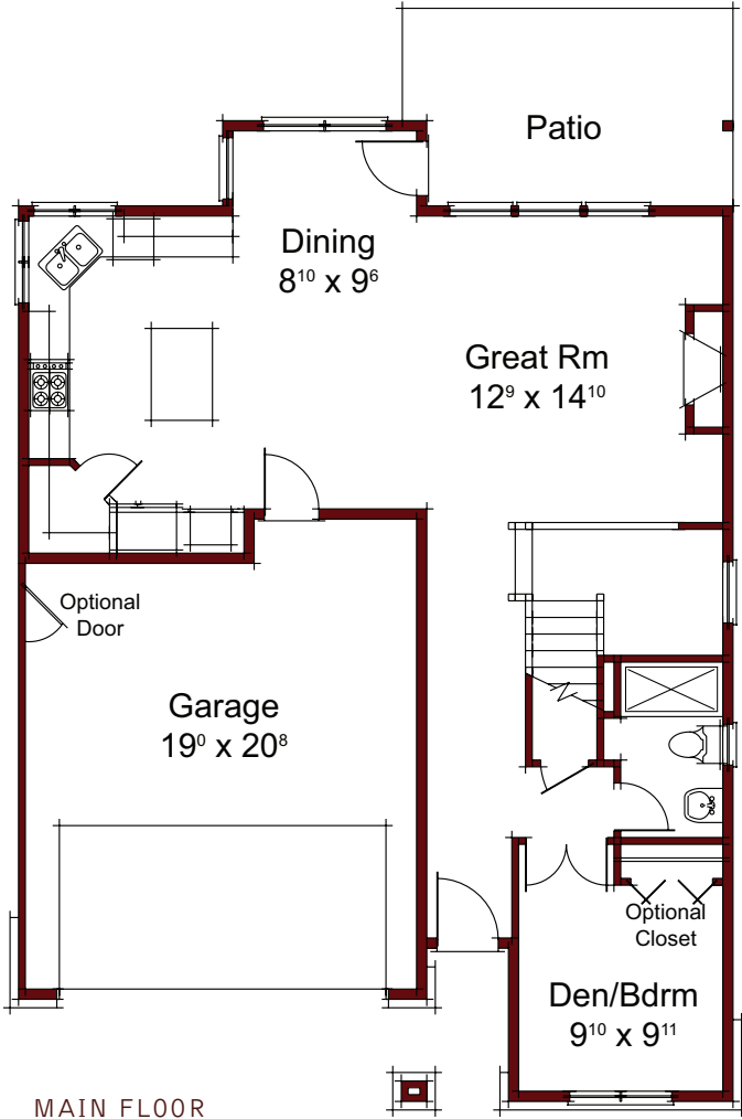
MAIN FLOOR
